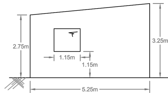
SIDE ELEVATION
