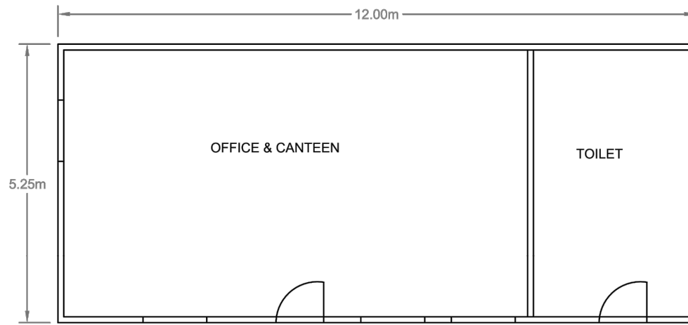
PERMANENT OFFICE & CANTEEN PLAN
